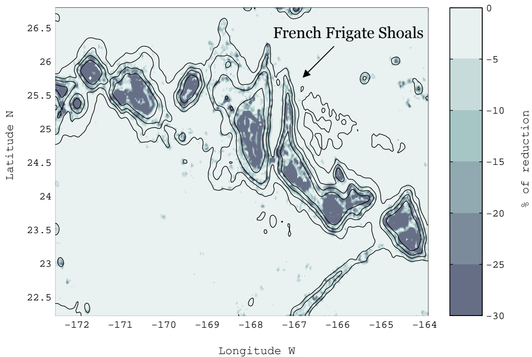
Reduction in tidal conversion as a result of smoothing
