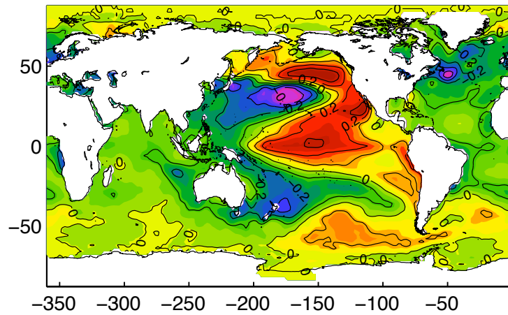
Regression of NPGO index with NOAA SSTa
