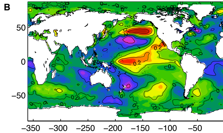
Regression of NPGO index with NOAA SSTa
