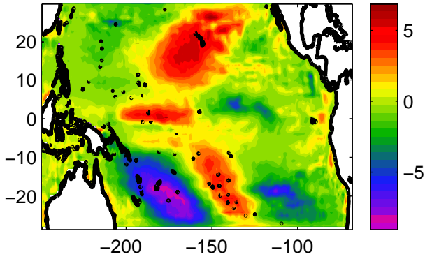
S-MODE SST EOF 3 6.4233%
