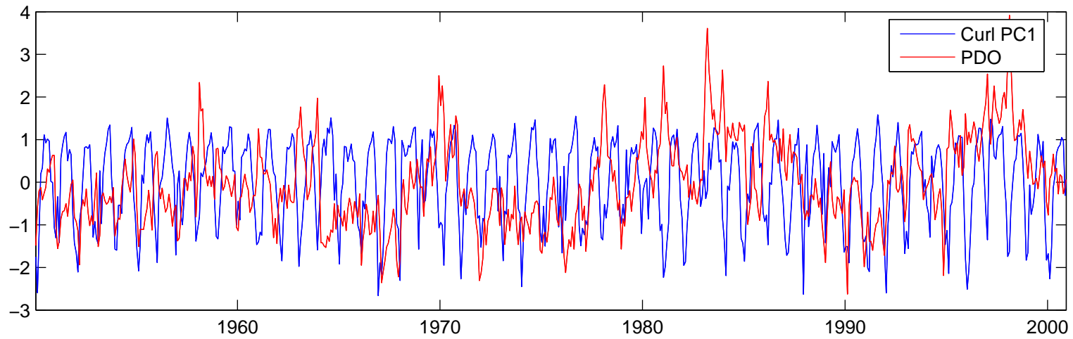
Wind stress curl PC 1
