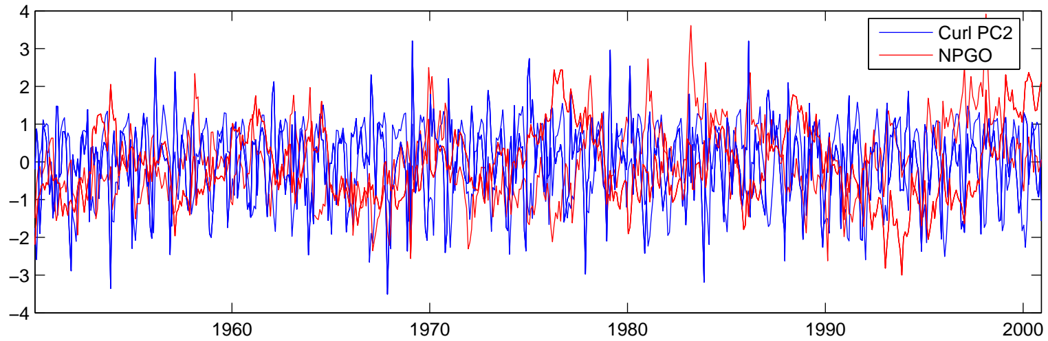
Wind stress curl PC 2
