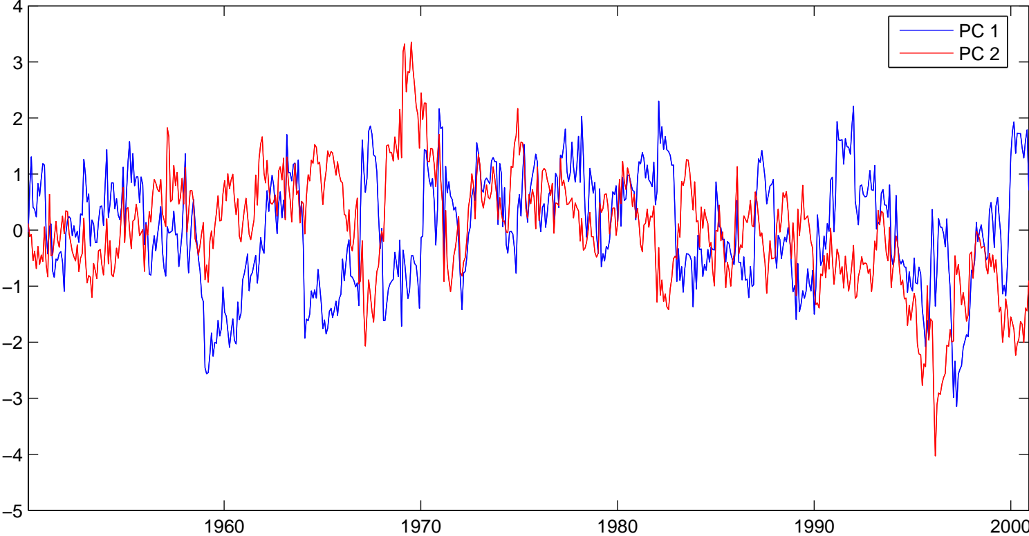
Zonal EOF
