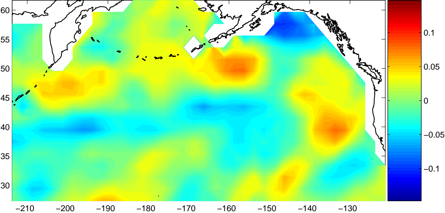
Regression NPGO – Wind stress curl
