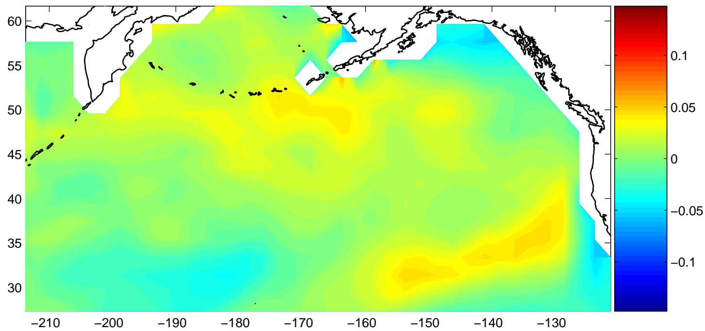
Regression GFDL SST – Wind stress curl
