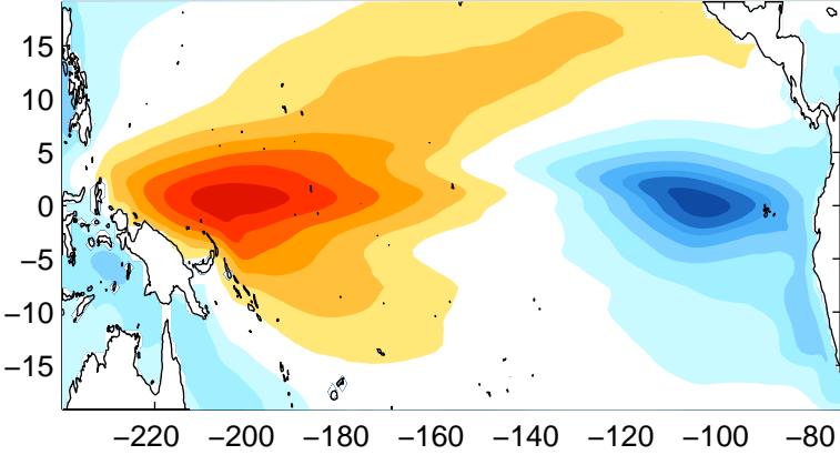
Tropical SST EOF-2
