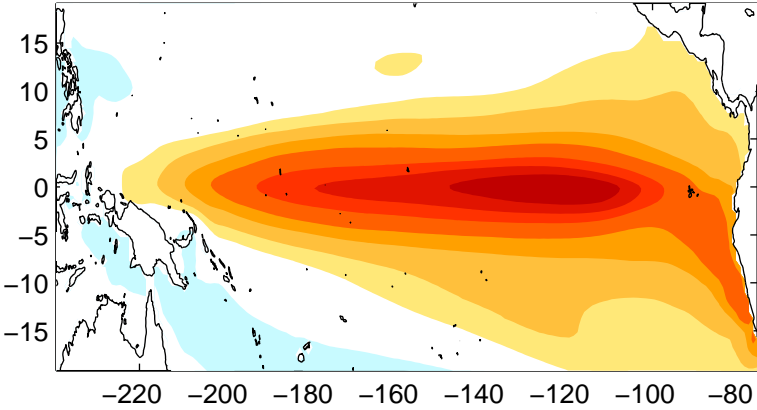
Tropical SST EOF-1
