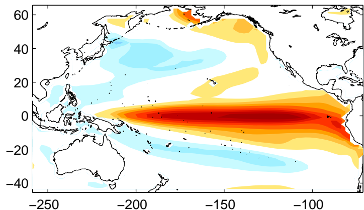
M4 Pacific SST EOF-1
