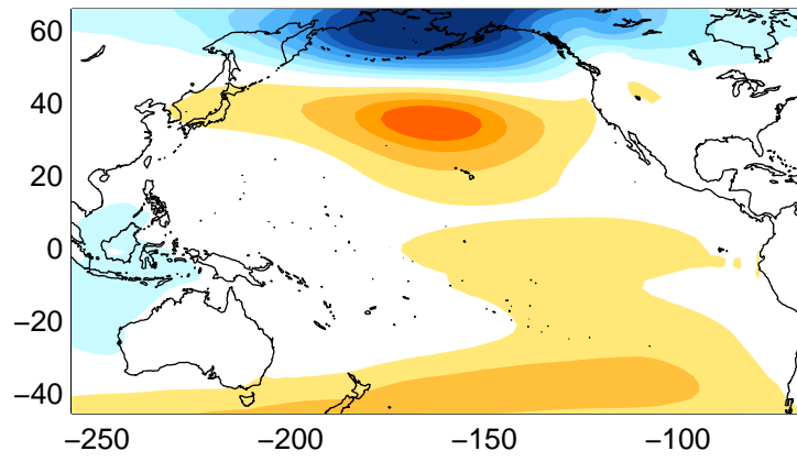
M3 SLP-SST Combined EOF Mode-2
