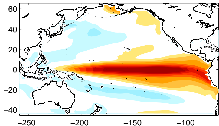
M3 Pacific SST EOF-1
