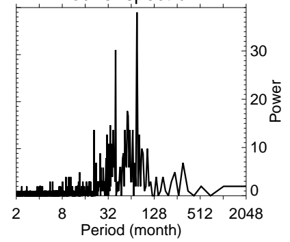
Fourier spectrum
