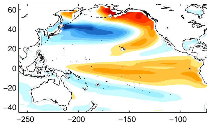
M3 North Pacific SST EOF-1
