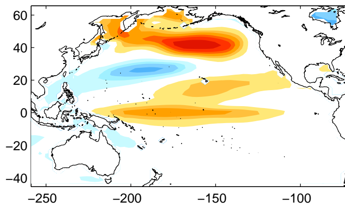
M3 North Pacific SST EOF-2
