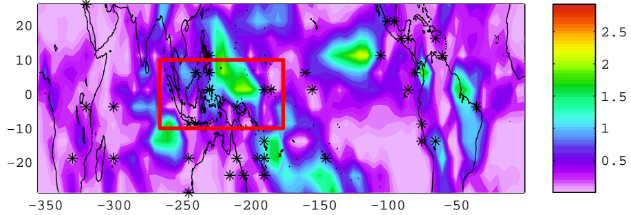
Source of information for Indian Ocean SST
