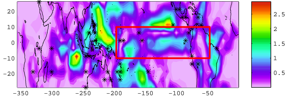
Source of information for Warm Pool SST
