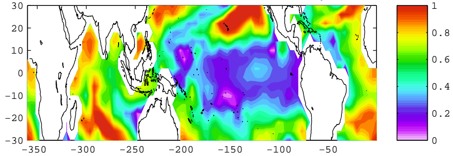
standardized error of network observability
