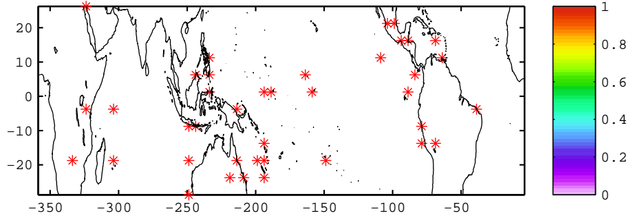
standard deviation ratio of true-reconstructed over SST std
