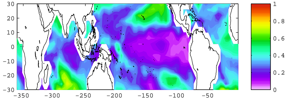
standardized error of network observability
